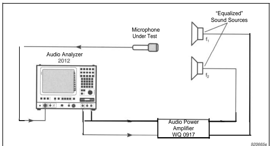
Fig. 23 Measurement setup for distortion measurements on microphones
