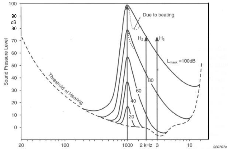
Fig. 6 Masking threshold for a pure tone in the presence of narrow band noise centered at 1 kHz (Zwicker, 1975). For a masking tone of 100 dB SPL, the 2nd Harmonic is masked for levels below 70 dB and the 3rd Harmonic is masked for levels below 60 dB SPL.
